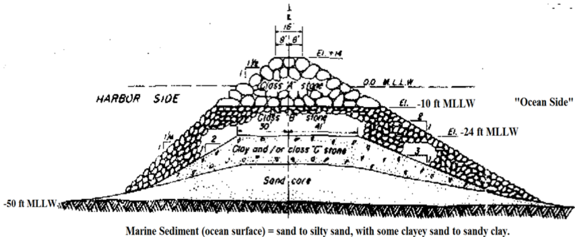
Figure 3.2: Profile of Long Beach Breakwater (USACE 2000, Condition Survey)
